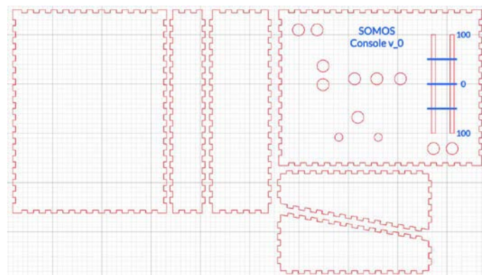
Figure 1. Laser-cutting design files for constructing the console enclosure
