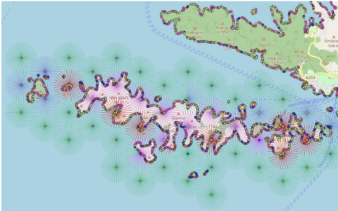
Figure 1. Ray-fetch analysis setup for the Pakleni Islands case study
