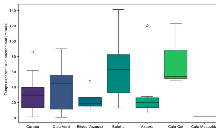
Figure 2. Waiting time (in minutes) of the tugs at the south entrance of the Port of Barcelona (data from 1/11/25-15/11/25)
