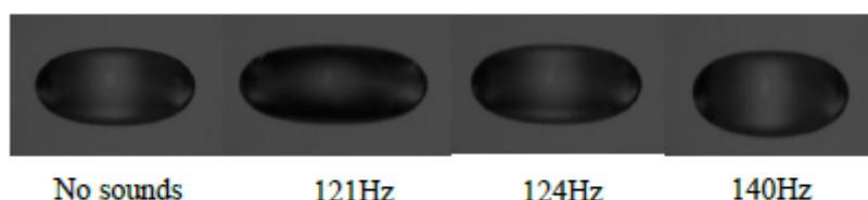
Figure 2. Droplet oscillation caused by sound waves from a speaker
