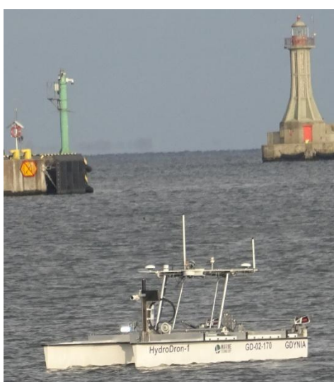
Figure 1. USV HydroDron-1 during measurements in the port of Gdynia.
