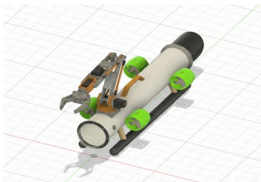
Figure 1. 3D Model of POSEIDON With Robotic Arm for underwater hull/structure maintenance.
