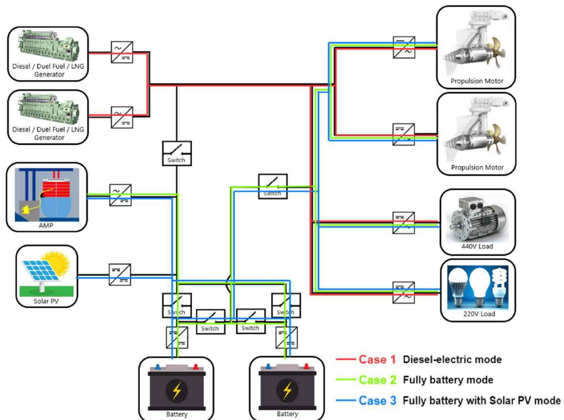
Figure 1. Concept design scenarios for a case ship
