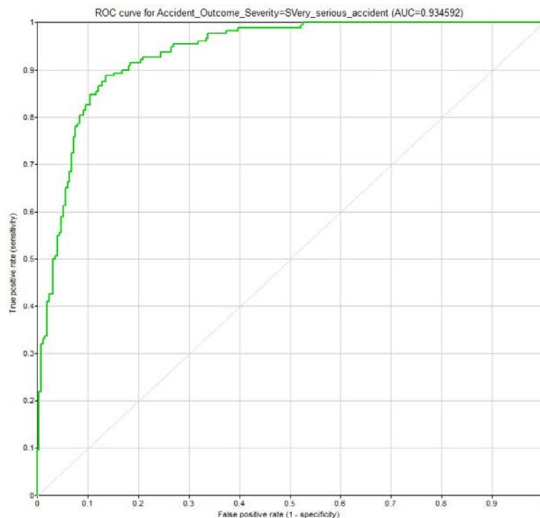
Figure 1. Validation Metrics for the state Very Serious Accidents.
